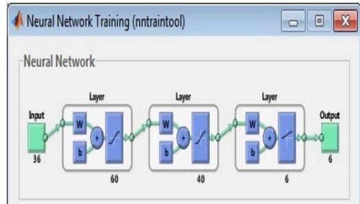
FIG.8 FEED FORWARD NEURAL NETWORK CLASSIFIER
