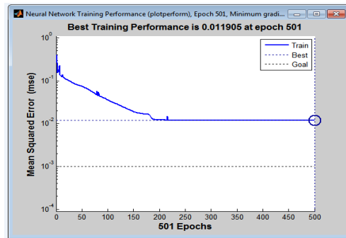
FIG.10 PERFORMANCE PLOT FOR DB1 WAVELET
