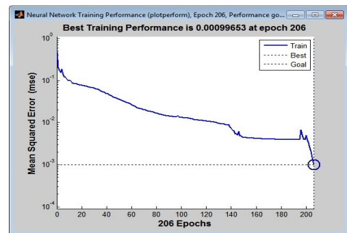
FIG.11. PERFORMANCE PLOT FOR ZERNIKE MOMENTS
