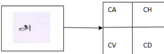
FIG.2 WAVELET DECOMPOSITION
